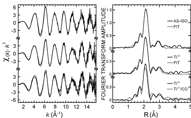
Figure 6. Ni k -space EXAFS and Fourier transforms for the ACDS \beta subunit.
